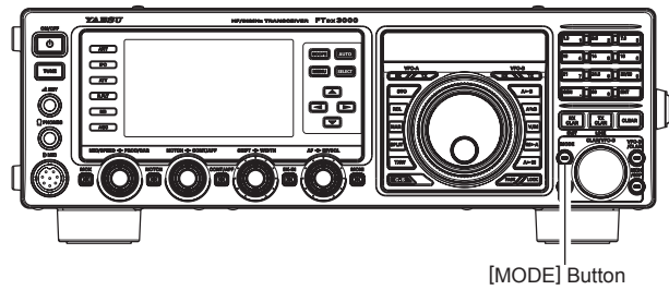
[MODE] Button
