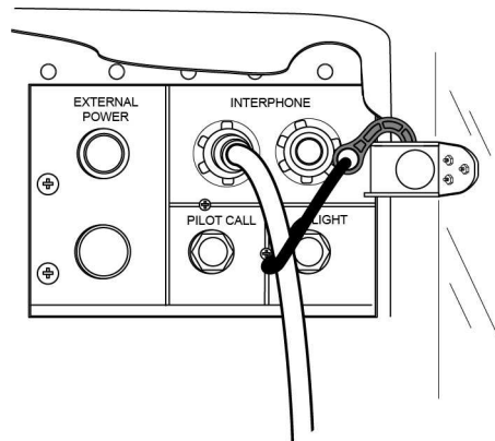
Figure 2: Example of hook attachment to aircraft
