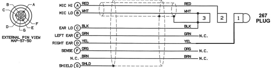
Figure 1: Cable Schematic (41035G-02)
